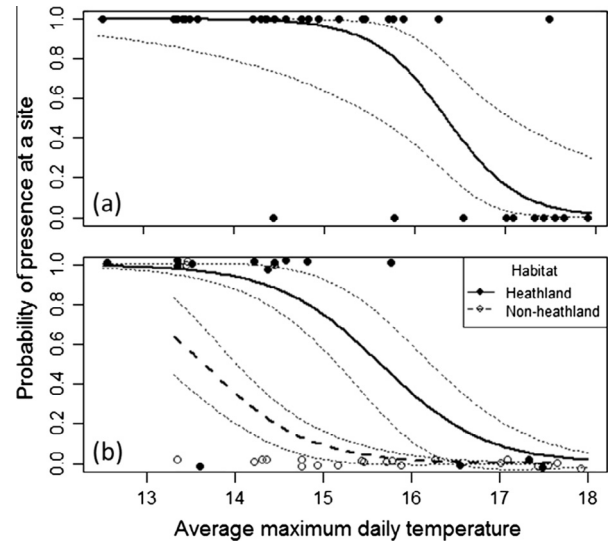
Fig. 3. (a) Probability of B. cryptarum presence at sites as a function of mean maximum daily temperature (°C) from March to August, and (b) of B. magnus presence as a function of mean maximum daily temperature (°C) on heathland (filled circles) and non-heathland habitat (non-filled circles). Bold lines represent the relationship between the presence of the species and the mean maximum daily temperature estimated from a generalised linear model. Small dashed lines represent 95% confidence intervals (CI) around this estimated relationship.
