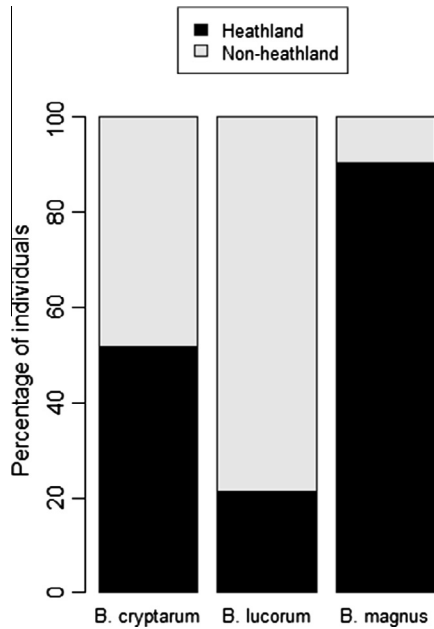
Fig. 2. Habitat use by all castes of B. lucorum , B. magnus and B. cryptarum , indicated by the percentage of bees caught in each habitat type, pooled for all sample sites.
