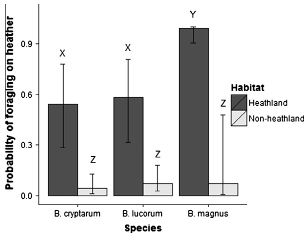
Fig. 4. The probability of individuals (queens and workers) of each taxa foraging on Calluna vulgaris , Erica tetralix or Erica cinerea compared to all other plant species, according to habitat type. Probabilities were estimated from a linear mixed effect model. Error bars show 95% confidence intervals. Probabilities with different letters are significantly different ( P < 0.001 ).
