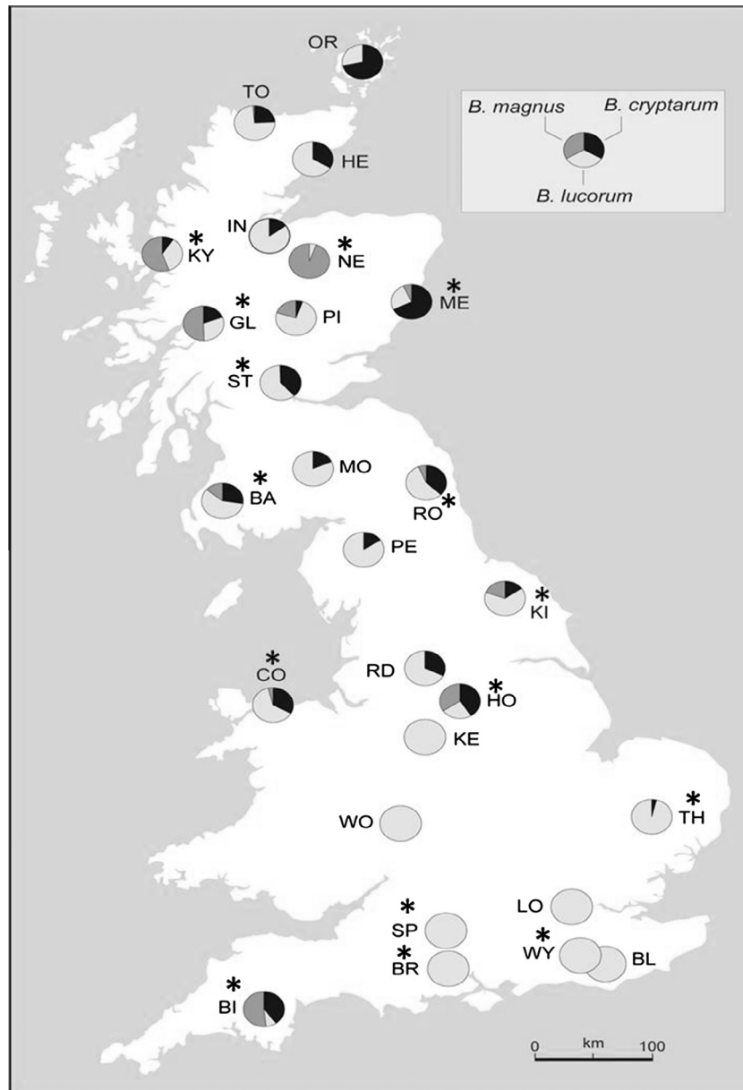
Fig. 1. The distribution of Bombus lucorum complex species across Great Britain. Sites marked with a * were sampled in 2011. The number of specimens identified per site, and habitat types sampled, are shown in Table S1.
